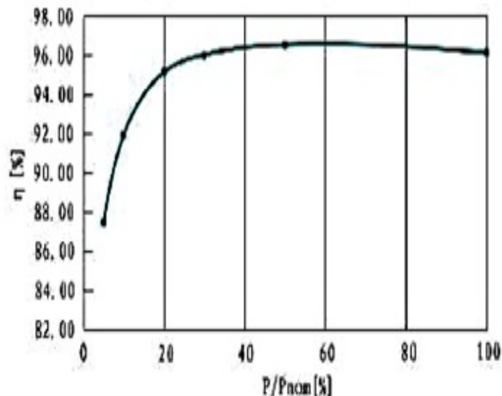
Efficiency curve
