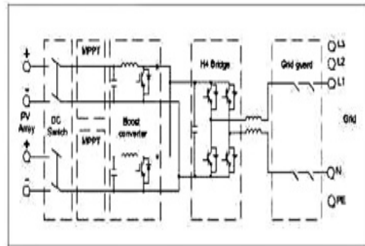
Electrical drawing
